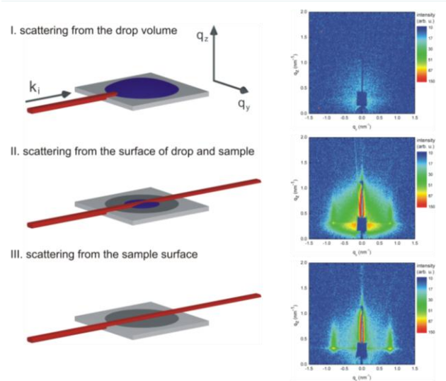
Fig. 4 - Scheme of the drying colloidal drop (left) and the corresponding GISAXS patterns taken in situ (right) in the inclined mode
