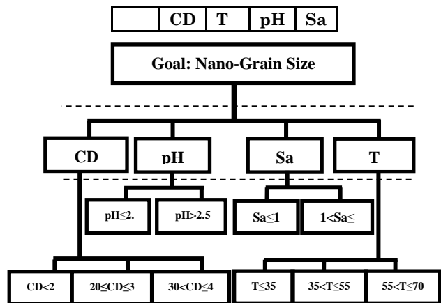
Fig. 2 – Hierarchy diagram of criteria for achieving the Cobalt coating smallest grain size
